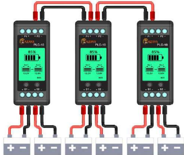
④ 6PCS Batteries Connect
