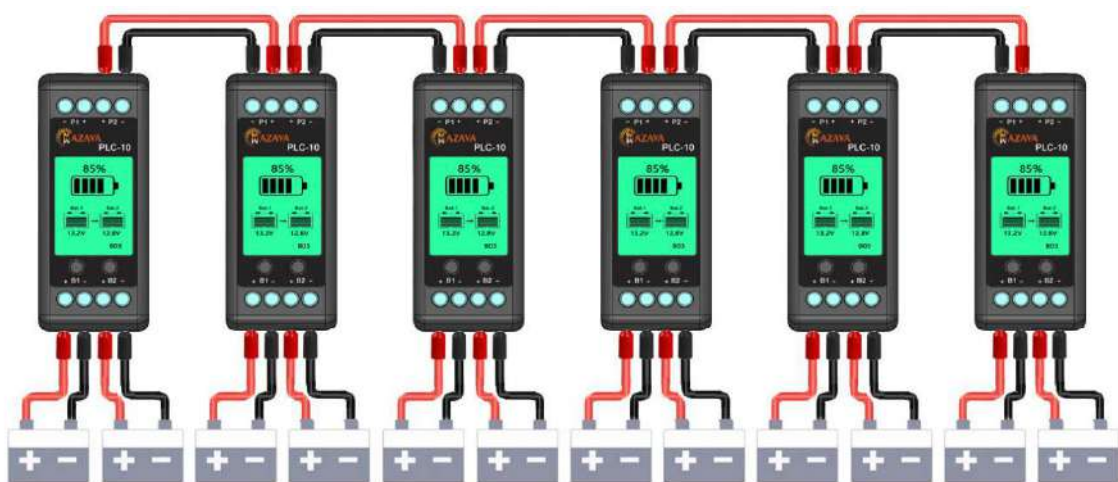
⑦ 12PCS Batteries Connect
