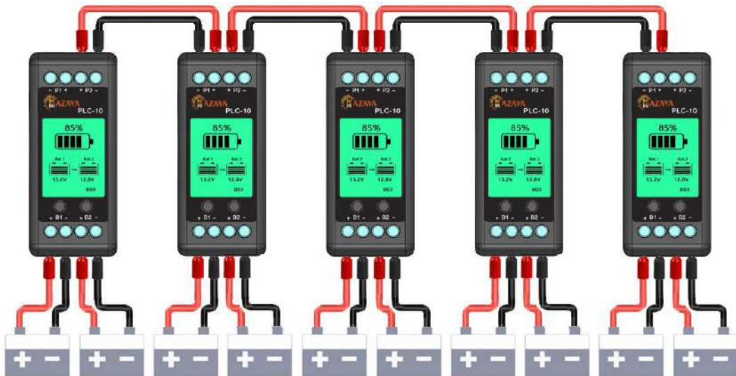
⑥ 10PCS Batteries Connect
