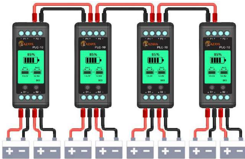
⑤ 8PCS Batteries Connect
