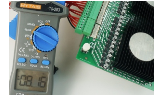
Monitor the equalizing current real time with a digital clamp meter
