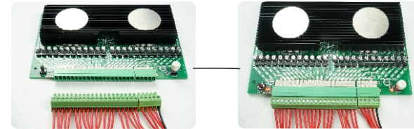
24S cable diagram: Black cable (terminal negative) connection B-, other cables are connected in line sequence.
