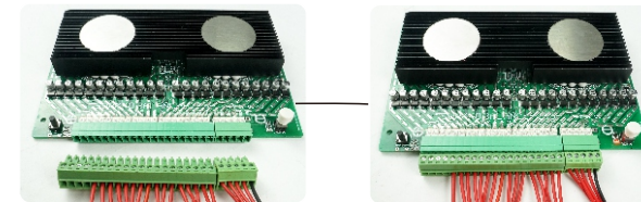
20S cable diagram: If connect 20S battery, the extra space in the back is not connected
