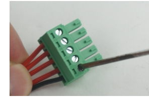
Connect the wire to the socket of 3.81 and pay attention to the locking screw
